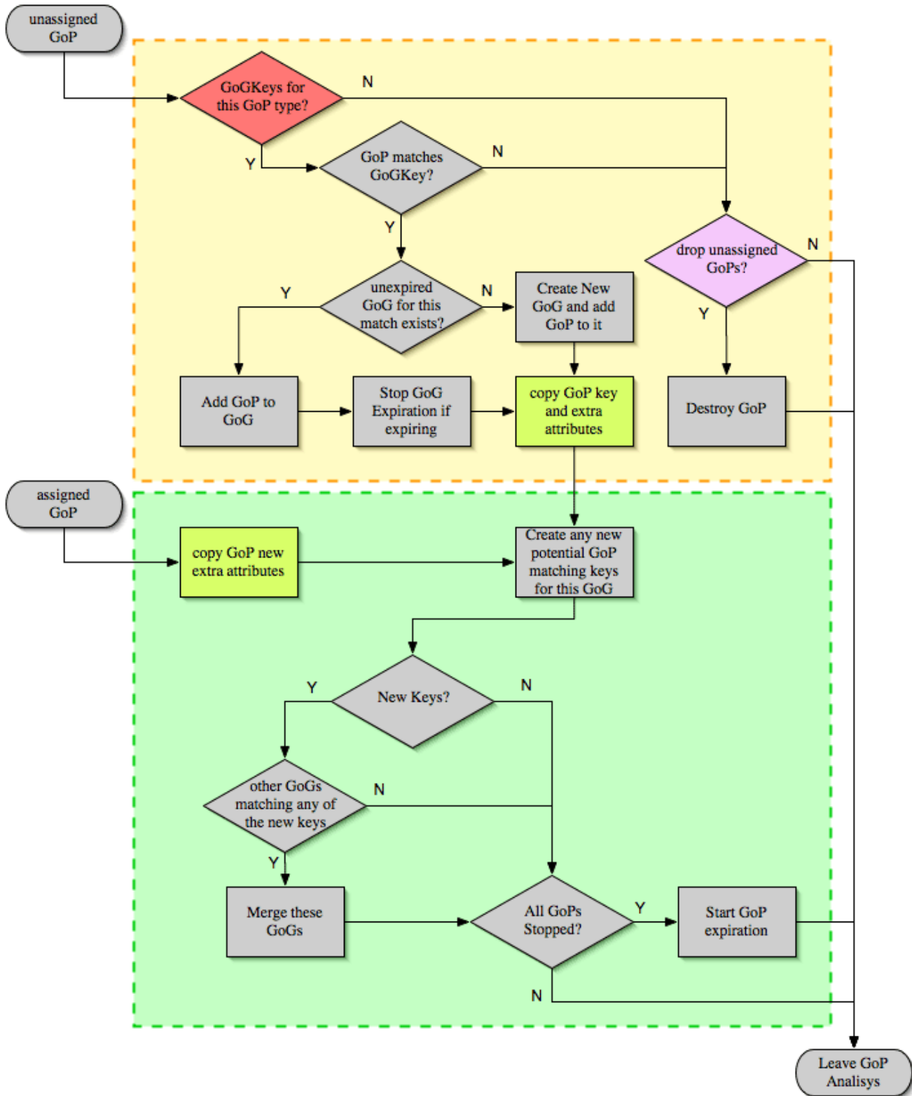
Figure 150. Grouping GOPs (GOG) flowchart
